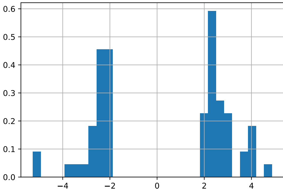
RELIANCE.NS Tail Zoom (Daily)
