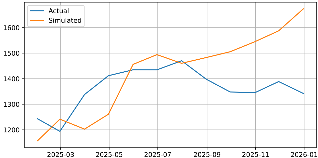
ICICIBANK.BO 2025 Simulation (Monthly)
