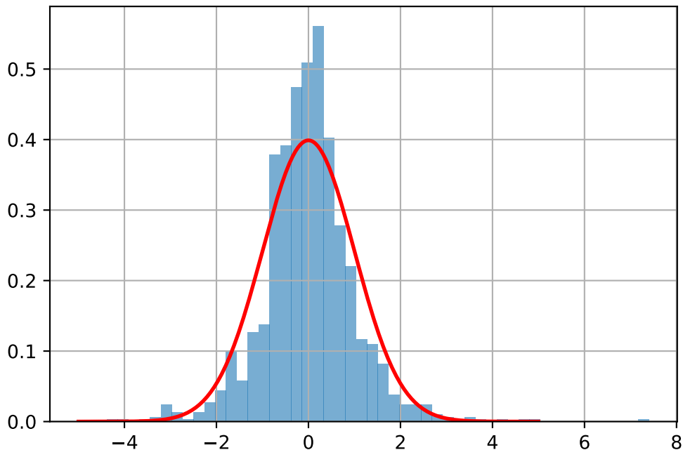
COFORGE.BO Arithmetic Normalized (Daily)
