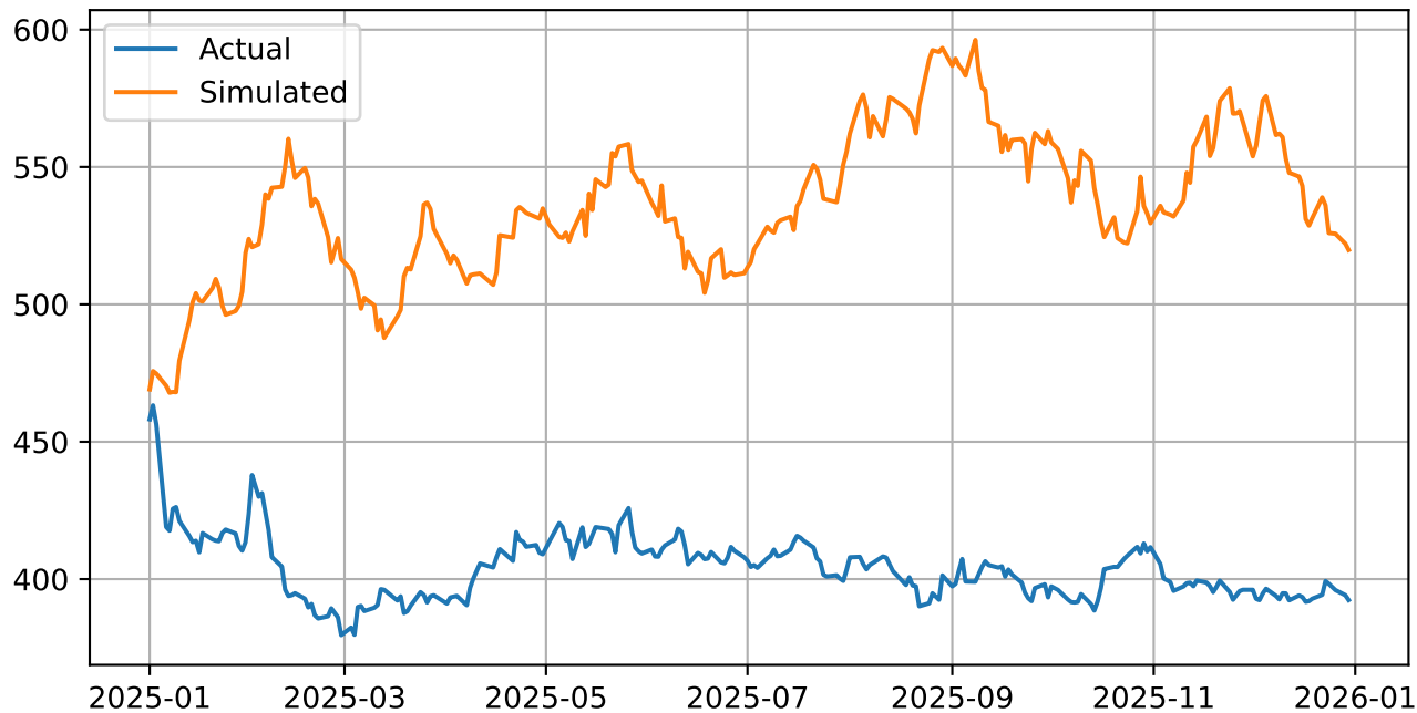
ITC.BO 2025 Simulation (Daily)
