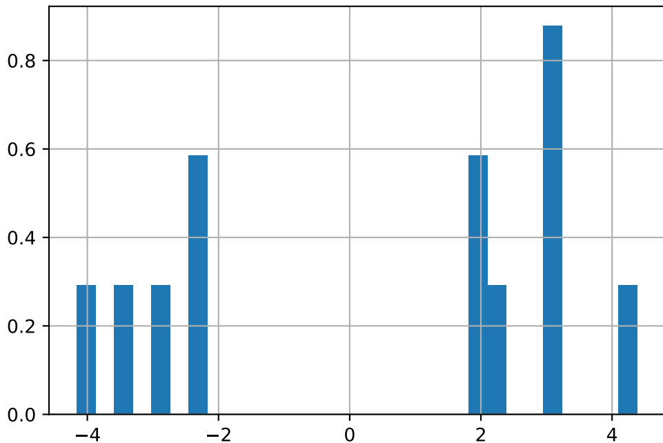
DEEPAKNTR.BO Tail Zoom (Weekly)
