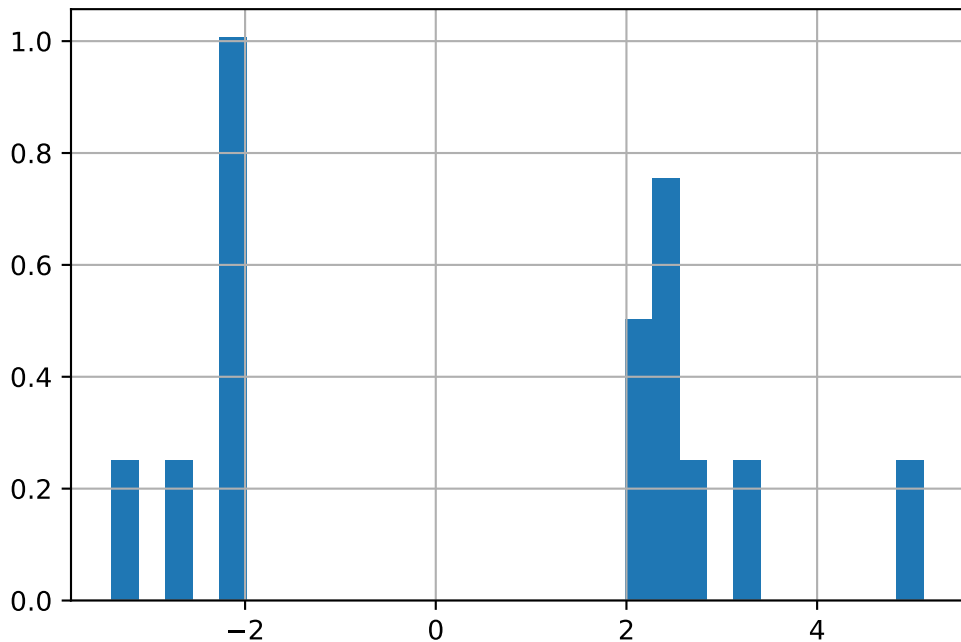
KOTAKBANK.BO Tail Zoom (Weekly)
